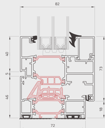
Sistema triplo vetro Triple glass system
