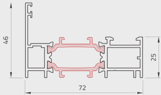
Telaio piano Flat frame
