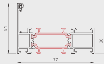
Telaio piano Flat frame
