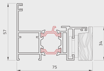
Telaio piano Flat frame
