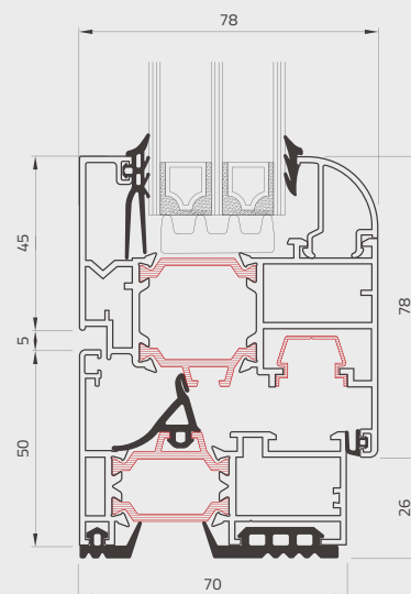
Sistema triplo vetro Triple glass system
